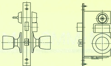
MHSE外観
