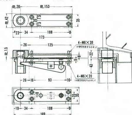
No.2 M56NF・M57NF逆付金具
