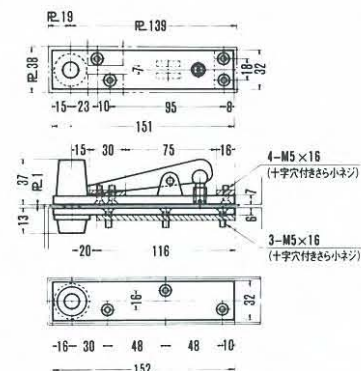
No.3 M54NF・M55NF
