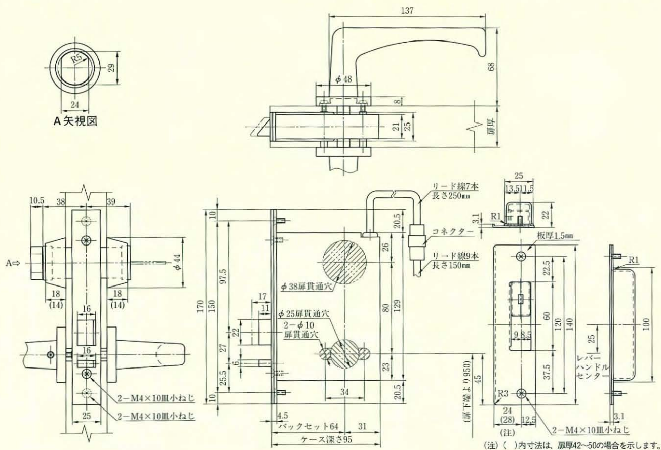
ALA-BL型(7線式)
