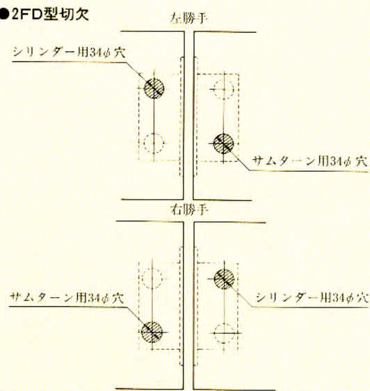
●2FD-EI型切欠
